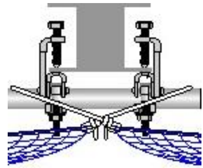
Figure 4. Correct use of a scaffold girder clamp
